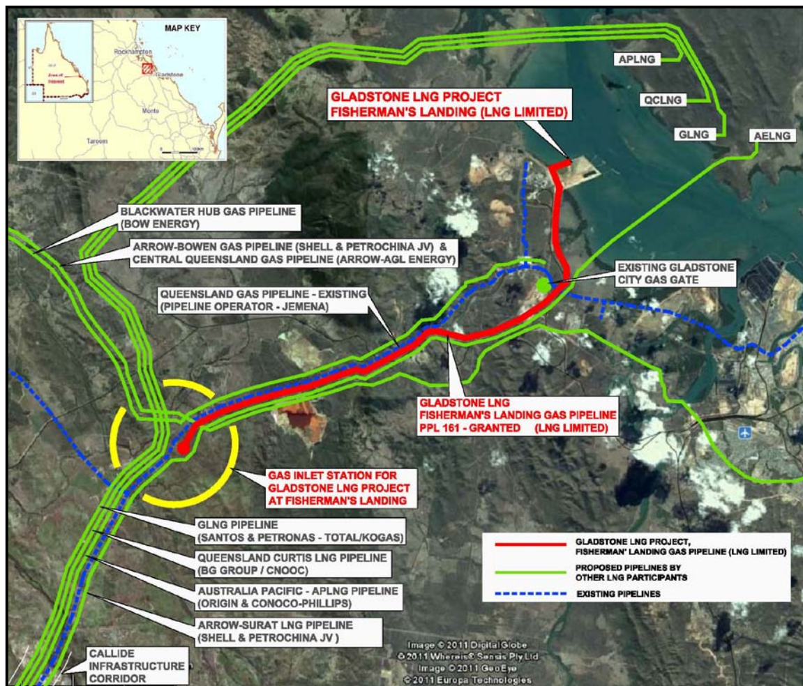
Gladstone LNG PPL 161 pipeline route and location of other existing and planned gas pipelines.
